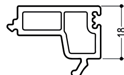
11330: Advance movable-fixed panel
