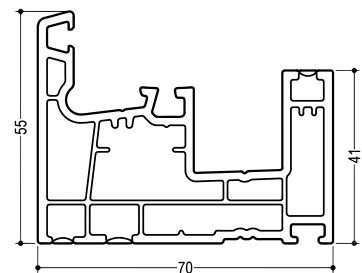
11330: Advance movable-fixed panel
